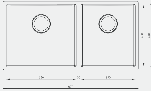
SSH-1B-01
