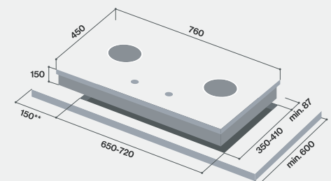
RB-3311S-GBC
