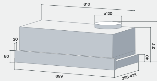
RH-TL95C-SSVR
