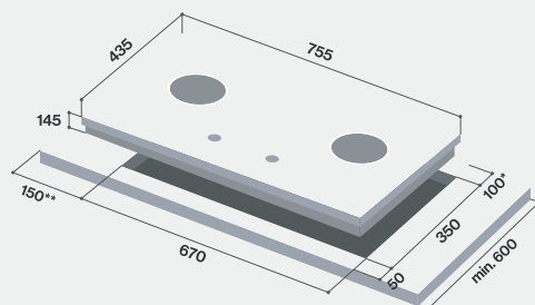
RB-L2620G-RM
