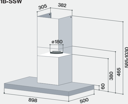
RH-C91B-SSW
