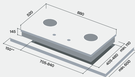
RB-782G
