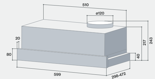
RH-TL65C-SSVR
