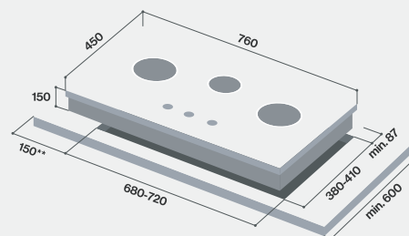
RB-3312S-GBC
