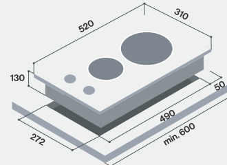
RB-3312S-GBC
