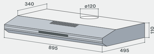
RH-S65A-SSVR
