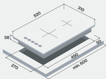
RB-3022H-CB
