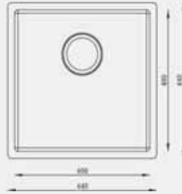
SSH-1B-01
